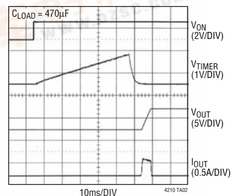
Power-Up Sequence
