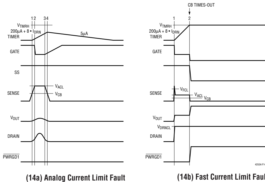
Figure 14. Current Limit Behavior (All Waveforms are Referenced to V_{EE} )
