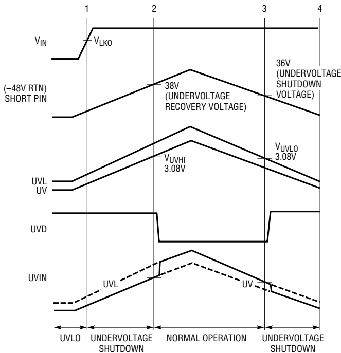
(2a) Undervoltage
