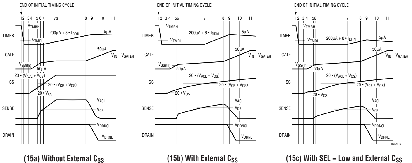
Figure 15. Soft-Start Timing (All Waveforms are Referenced to V_{EE} )
