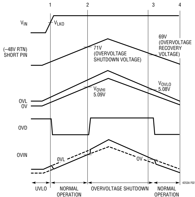
(2b) Overvoltage
