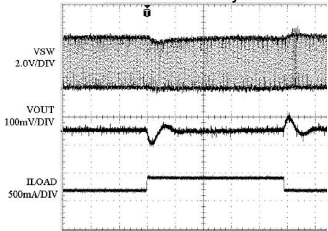
Load Transient Response PWM Mode Only
