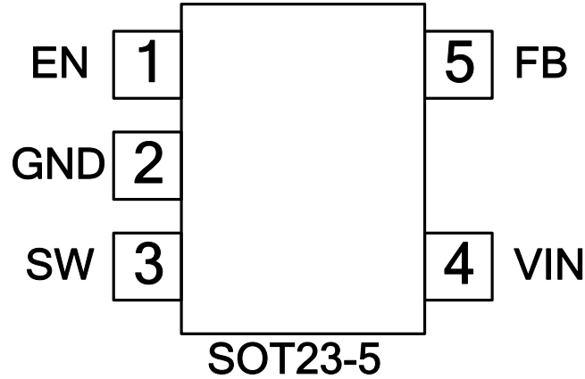
Figure 2: Pin Configuration
