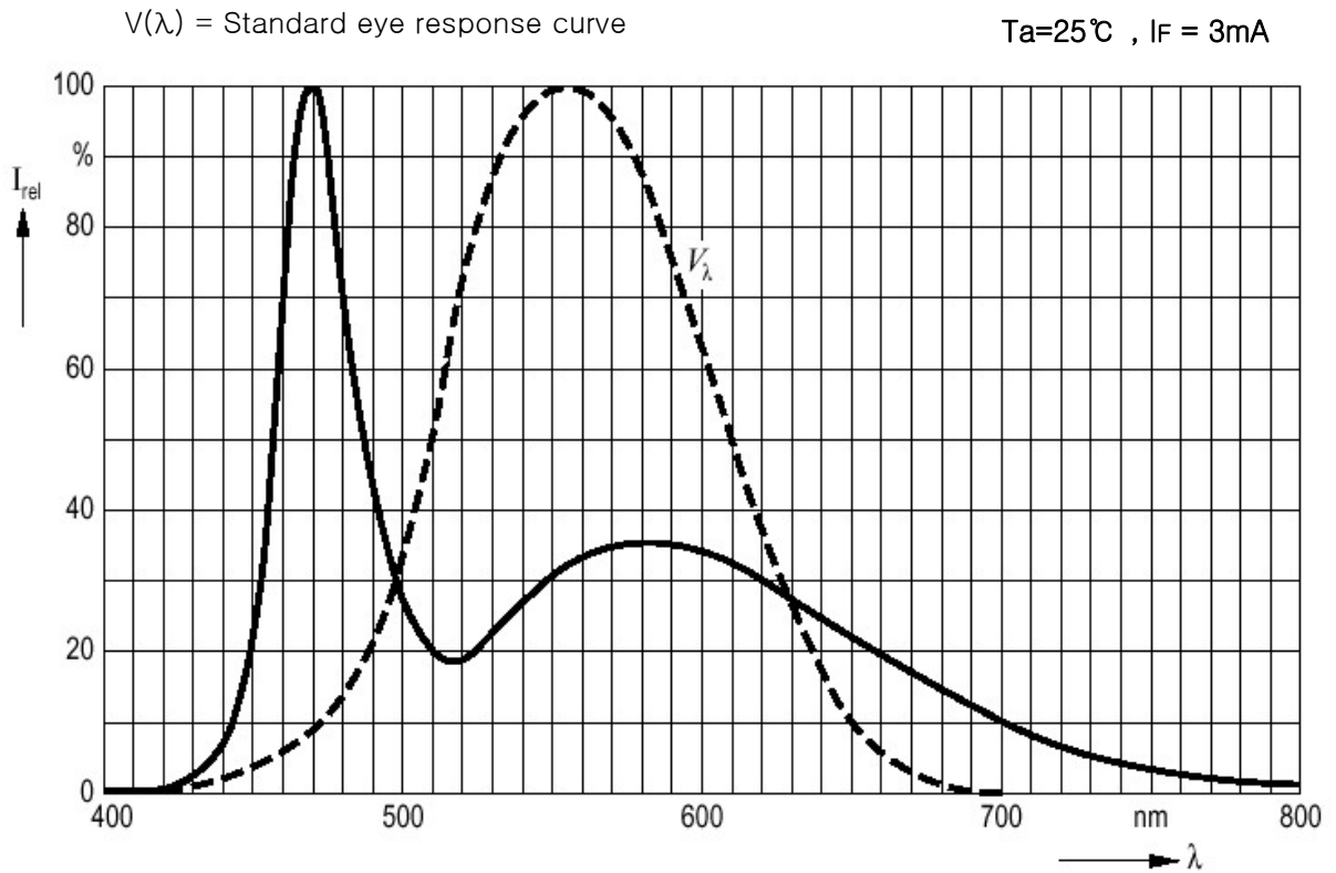
Fig. 5 Relative Spectral Emission
