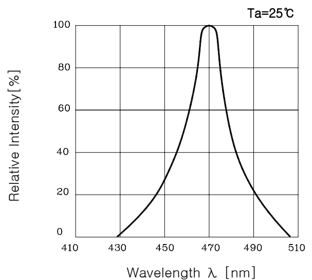
Fig. 4 Spectrum Distribution
