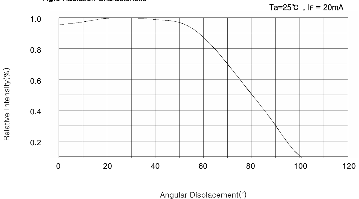
Fig.6 Radiation Characteristic
