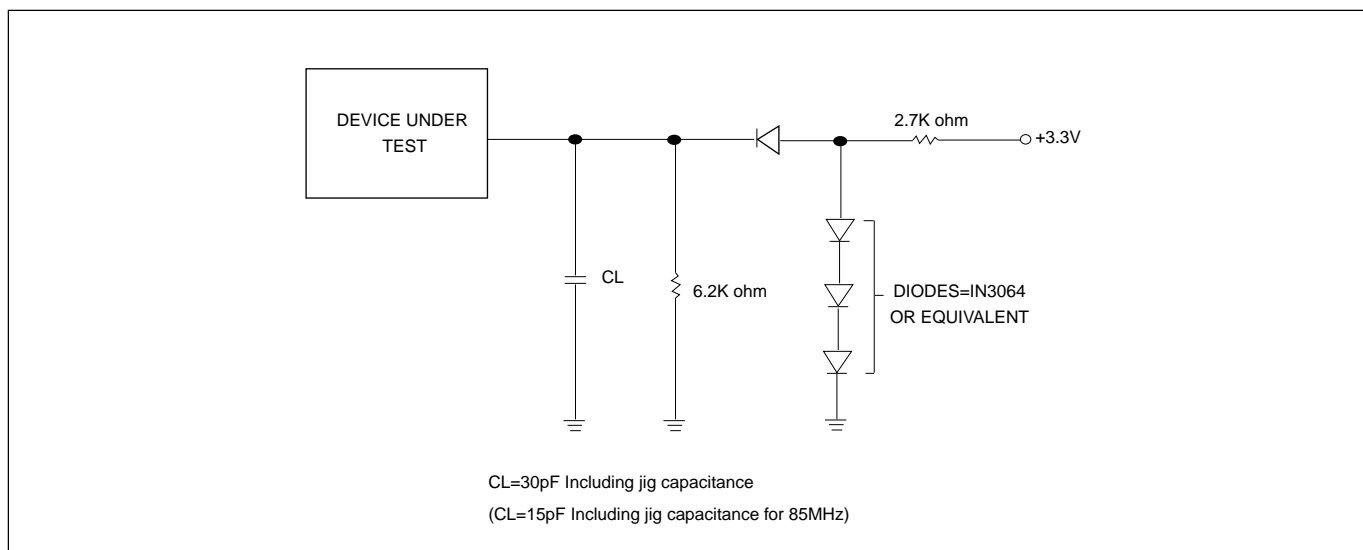
Figure 6. OUTPUT LOADING
