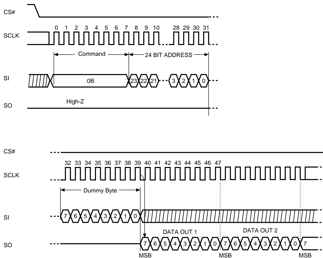
Figure 17. Read at Higher Speed (FAST_READ) Sequence (Command 0B)
