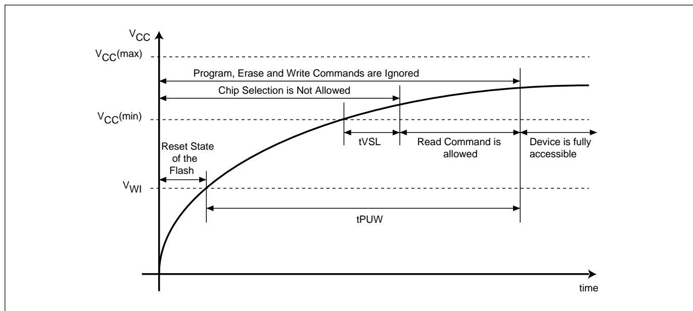
Figure 26. Power-up Timing
