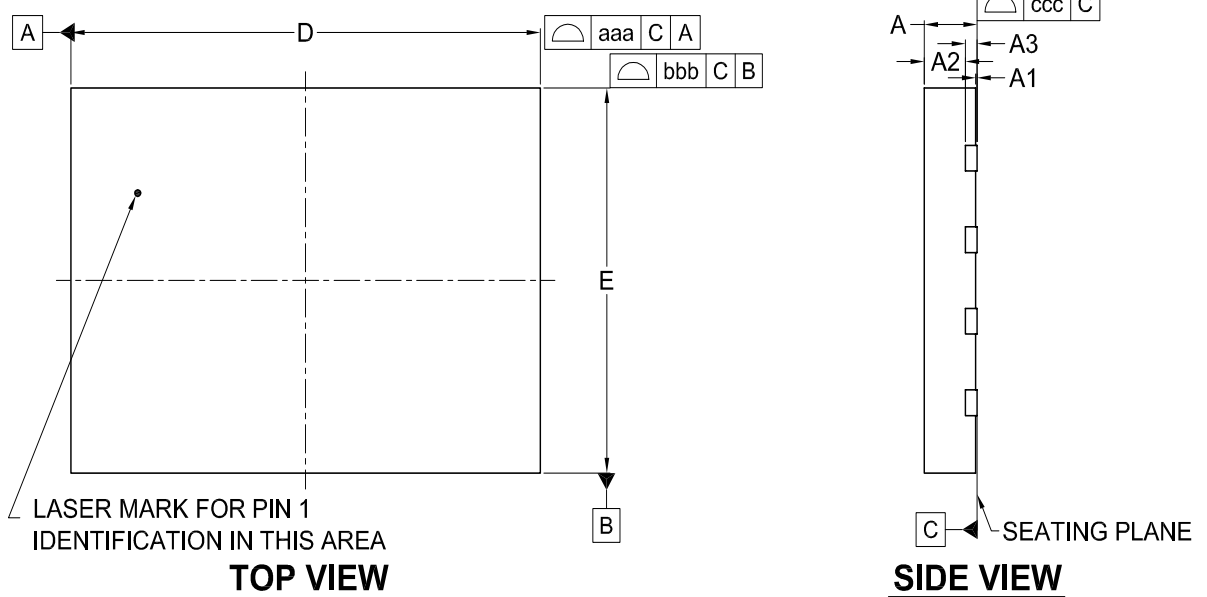
Title: Package Outline for SON 8L (8x6x1.0MM, LEAD PITCH 1.27MM)
