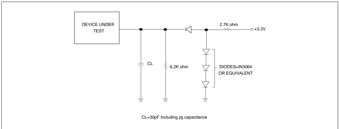
Figure 7. OUTPUT LOADING
