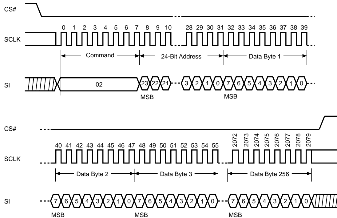
Figure 18. Page Program (PP) Sequence (Command 02)
