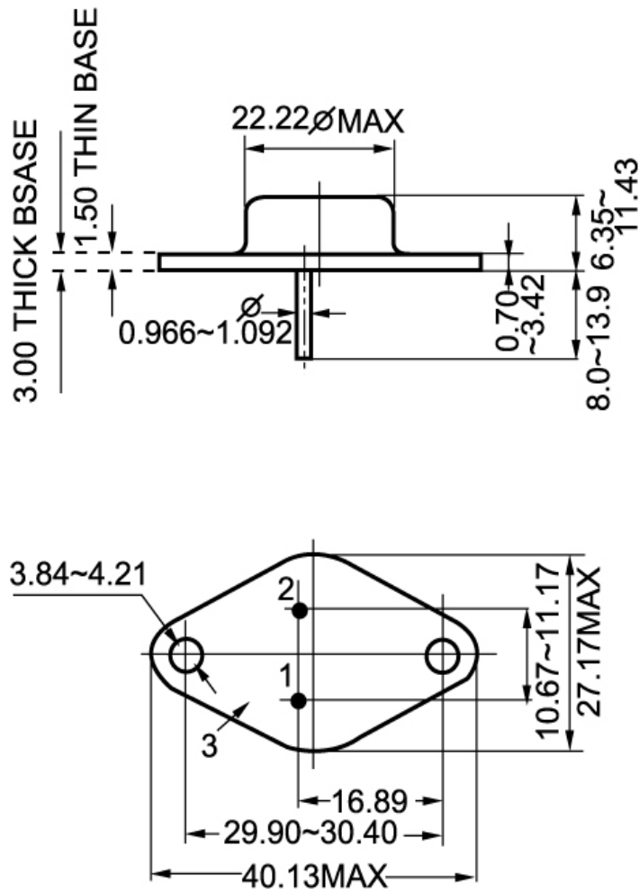
Fig.2 outline dimensions
