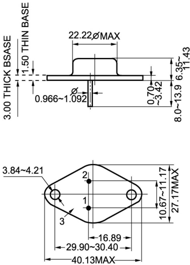
Fig.2 Outline dimensions
