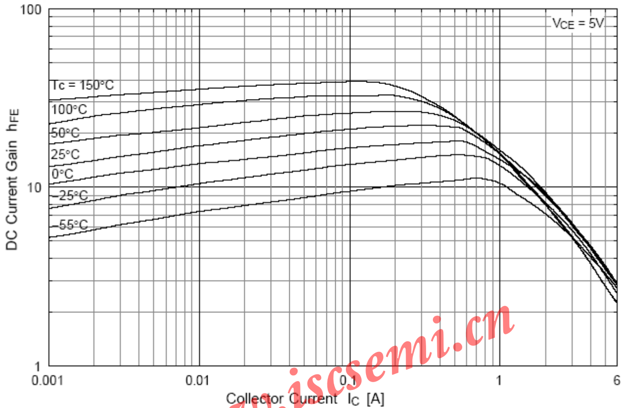
h_{FE} - I_C Characteristics
