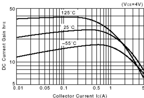
Fig.7 DC current Gain
