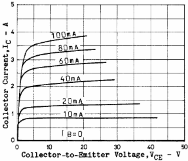
Fig.3 Static Characteristic
