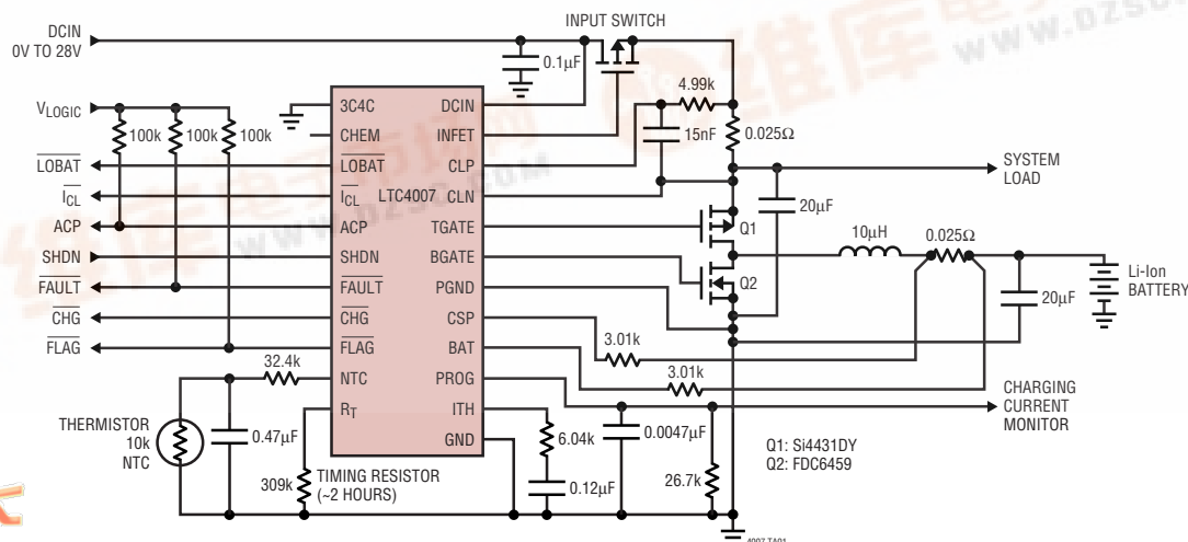
12.6V, 4A Li-Ion Battery Charger
