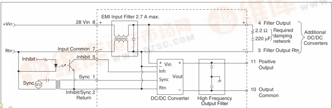
FIGURE 1: FMTR TYPICAL INPUT INTERFACE APPLIES TO SINGLES AND DUALS (SHOWN WITH SINGLE OUTPUT)
