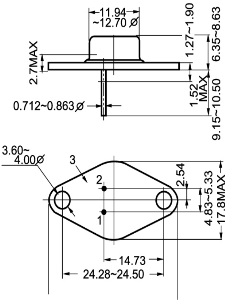
Fig.2 Outline dimensions
