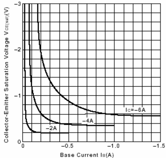
Fig.4 V_{CE(sat)}-I_B Characteristics
