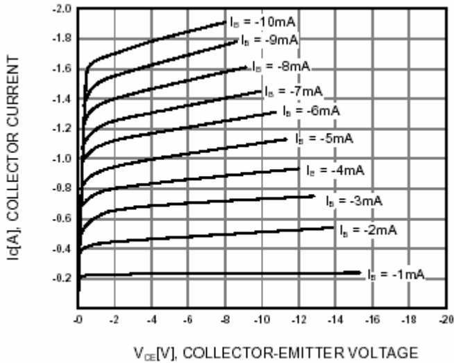
Fig.3 Static Characteristic
