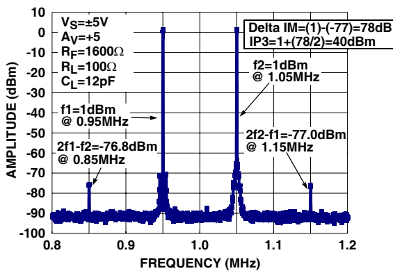
FIGURE 35. THIRD ORDER IMD INTERCEPT (IP3)
