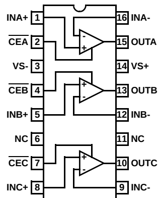
EL5302 (16 LD QSOP) TOP VIEW
