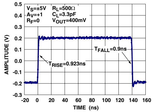
FIGURE 32. SMALL SIGNAL STEP RESPONSE_RISE AND FALL TIME
