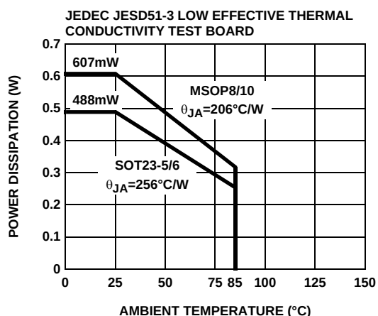
FIGURE 39. PACKAGE POWER DISSIPATION vs AMBIENT TEMPERATURE
