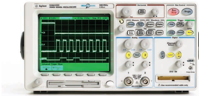
Figure 7. Trigger on data patterns within a SPI frame.
