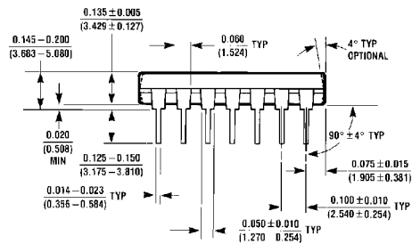
14-Lead Molded Dual-In-Line Package (N) Order Number DM74LS02N Package Number N14A
