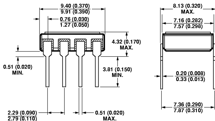
8 Pin DIP Through Hole, 1 and 2 Channel
