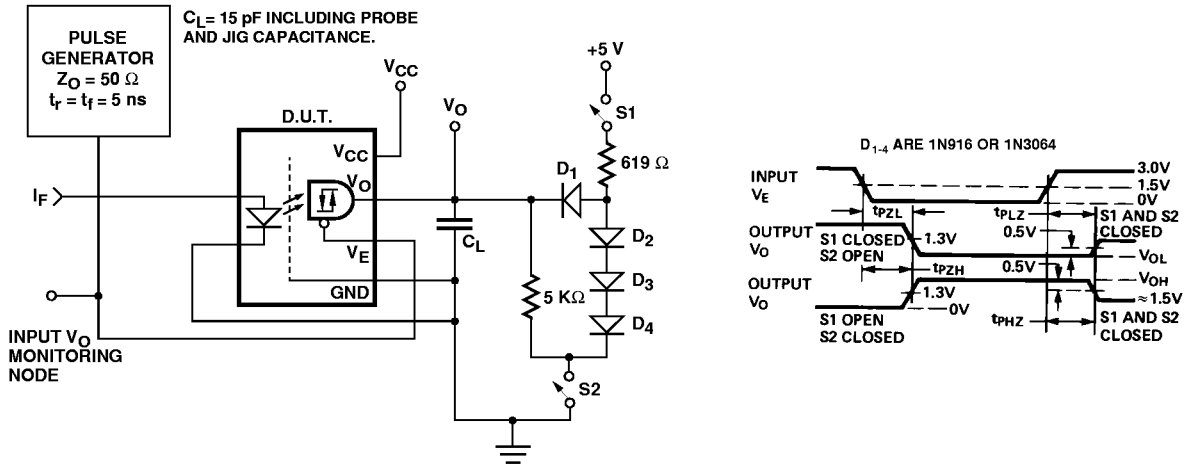
Figure 8. Test Circuit for t_{PHZ} , t_{PLZ} , t_{PLZ'} and t_{PZH} .
