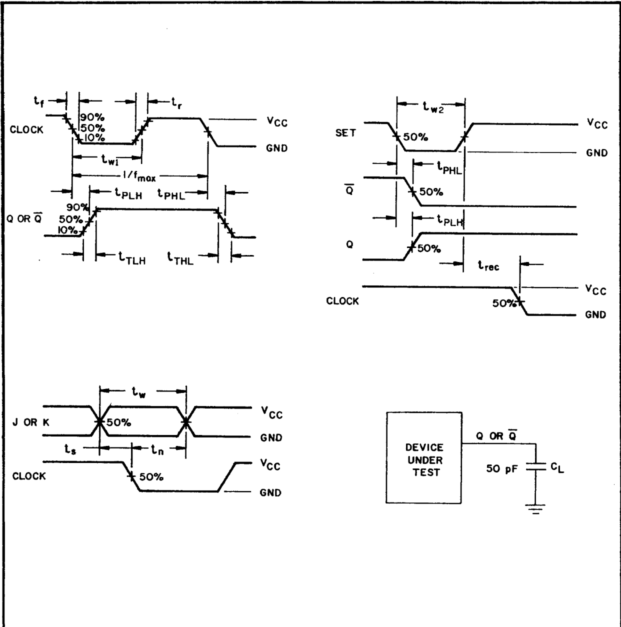
FIGURE 3. Test circuit and switching waveforms.
