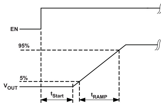
Figure 20. Soft Start
