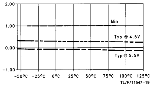
t PLH vs Temperature (T A )
