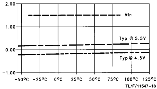
t HOLD LOW vs Temperature (T A )
