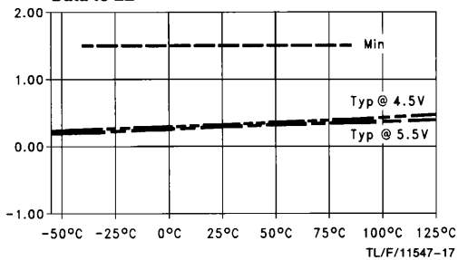
t HOLD HIGH vs Temperature (T A )
