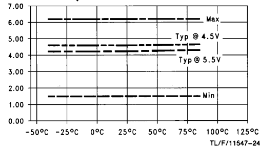
t pZL vs Temperature (T A )
