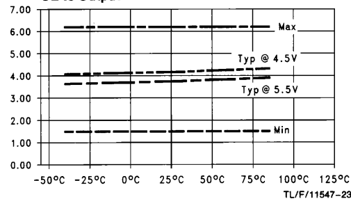
t pZH vs Temperature (T A )
