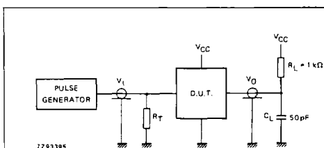
Fig. 7 Test circuit (open drain)
