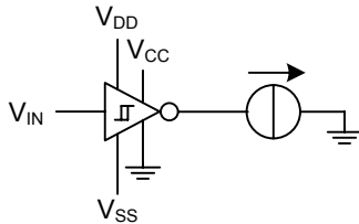
Figure 4. I_{OS}
