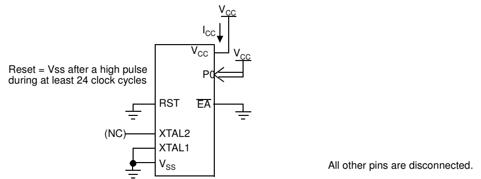
Figure 5. I_{CC} Test Condition, Power-down Mode
