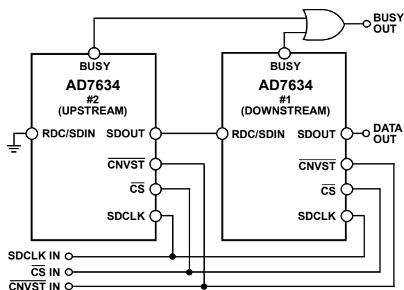
Figure 43. Two AD7634 Devices in a Daisy-Chain Configuration
