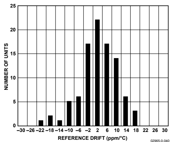
Figure 18. Reference Voltage Temperature Coefficient Distribution (100 Units)
