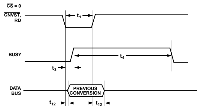
Figure 30. Slave Parallel Data Timing for Reading (Read during Convert)
