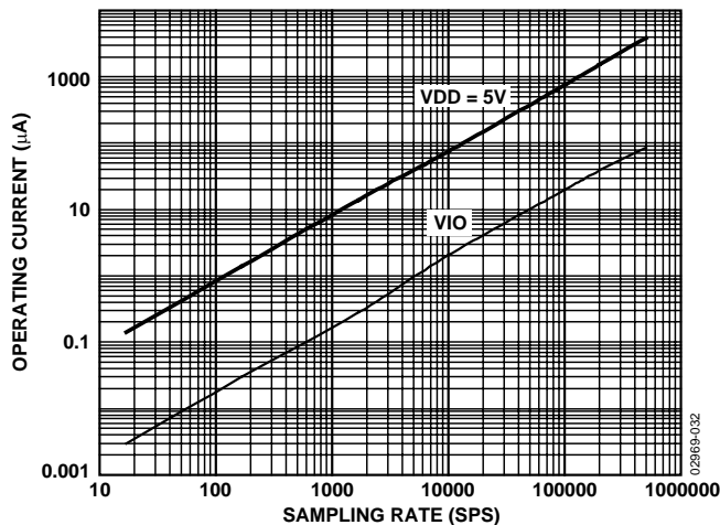
Figure 31. Operating Current vs. Sampling Rate
