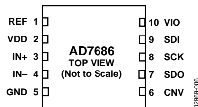
Figure 6. 10-Lead QFN (LFCSP) Pin Configuration
