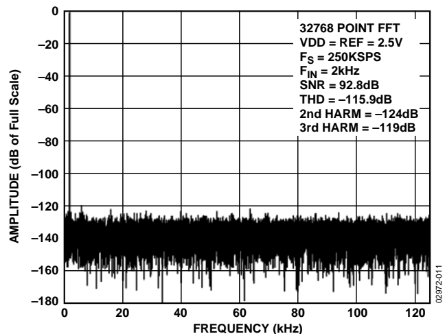
Figure 12. FFT Plot
