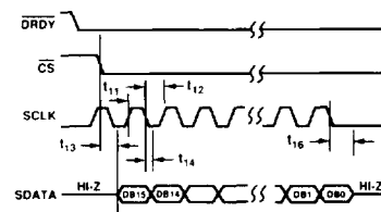
Figure 4b. SEC Mode Timing Diagram
