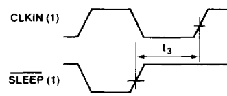
2b. SLEEP Mode Timing
