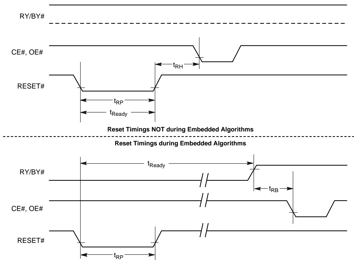
Figure 16. Reset Timings
