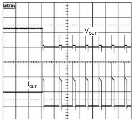
Ch1 : V_{OUT} , 1V/Div, DC Ch2 : I_{OUT} , 2A/Div Time : 50ms/Div
