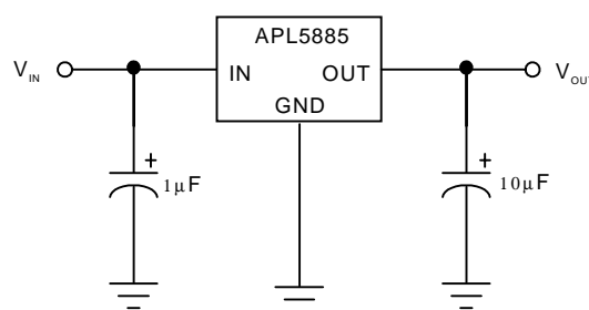
Fixed 1.8V, 2.5V and 3.3V Regulator
