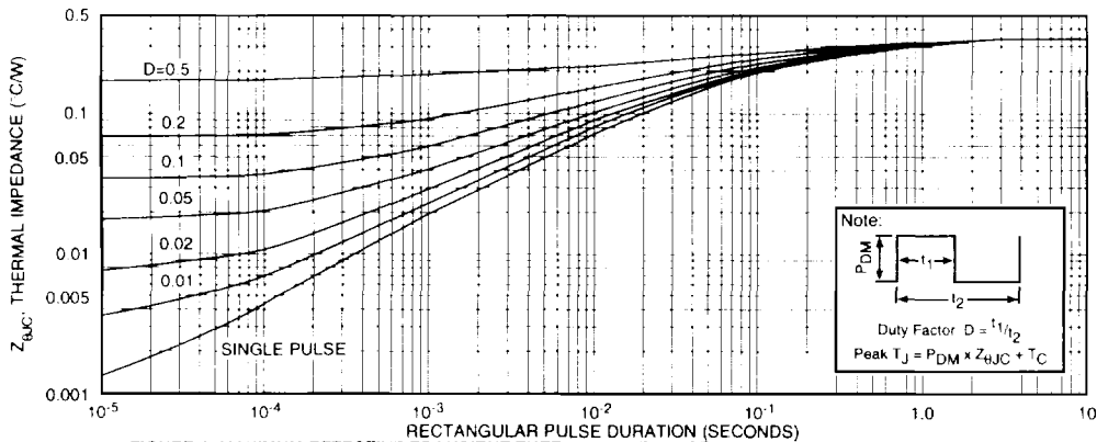
FIGURE 1. MAXIMUM EFFECTIVE TRANSIENT THERMAL IMPEDANCE, JUNCTION-TO-CASE vs PULSE DURATION Page 43
