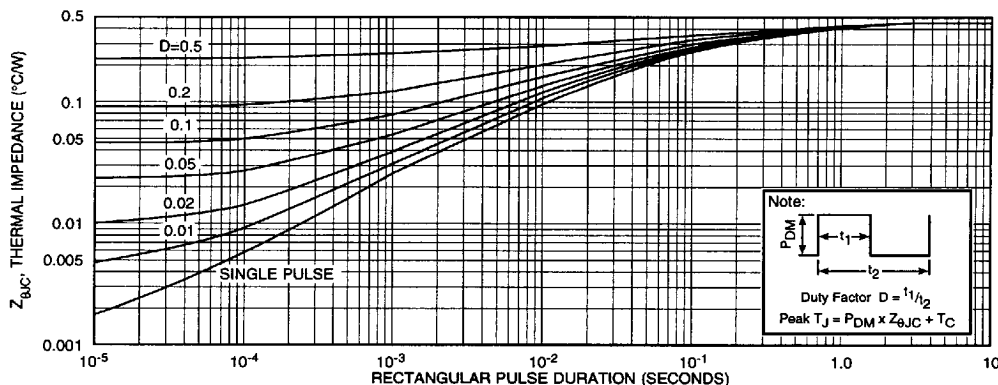
FIGURE 1, MAXIMUM EFFECTIVE TRANSIENT THERMAL IMPEDANCE, JUNCTION-TO-CASE vs PULSE DURATION Page 87
