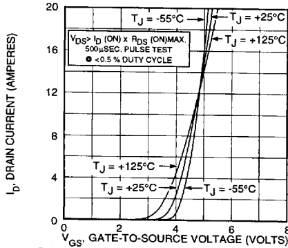
FIGURE 4, TYPICAL TRANSFER CHARACTERISTICS
