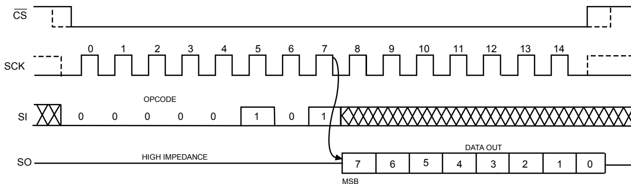
Figure 11. RDSR Timing
