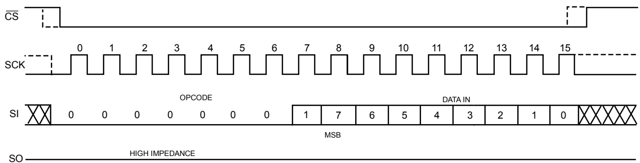
Figure 8. WRSR Timing
