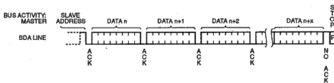
Figure 10. Sequential Read Timing
