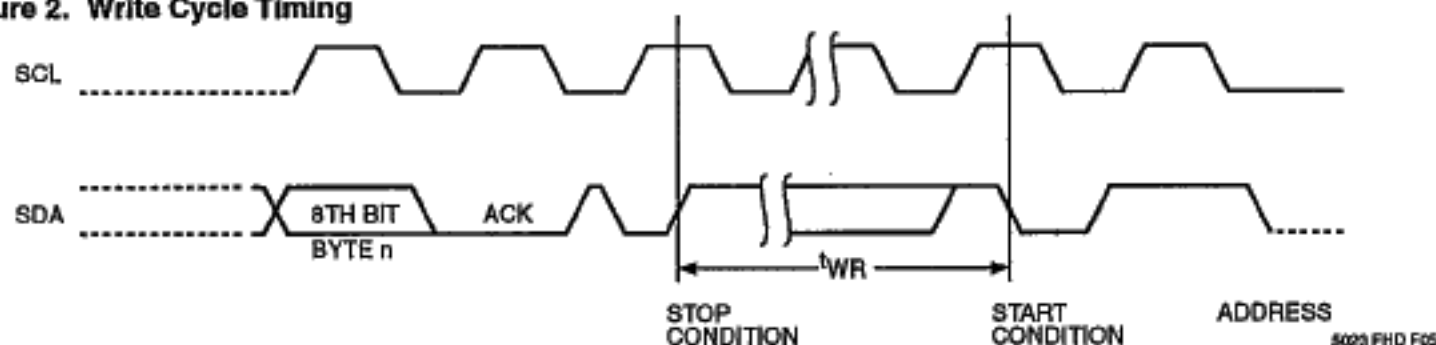
Figure 2. Write Cycle Timing
