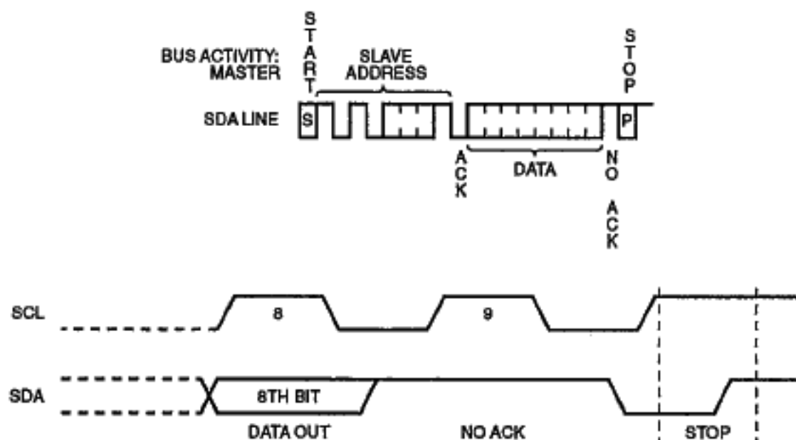
Figure 8. Immediate Address Read Timing
