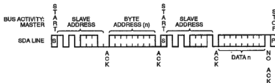
Figure 9. Selective Read Timing
