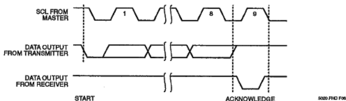
Figure 4. Acknowledge Timing
