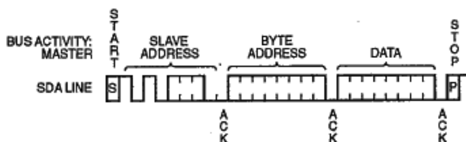
Figure 6. Byte Write Timing
