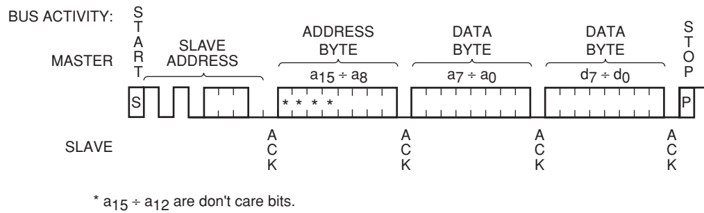
Figure 5. Byte Write Sequence
