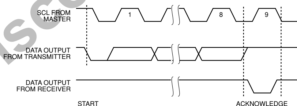
Figure 4. Acknowledge Timing
