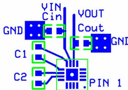
Figure 2. PCB Layout
