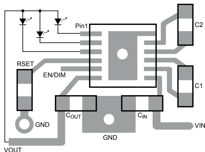
Figure 5. TDFN-12 Recommended Layout
