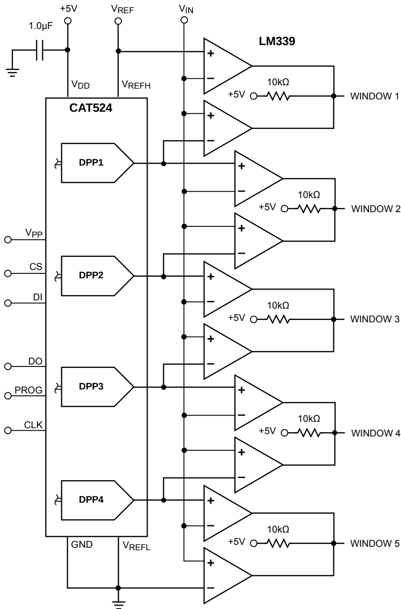
Staircase Window Comparator
