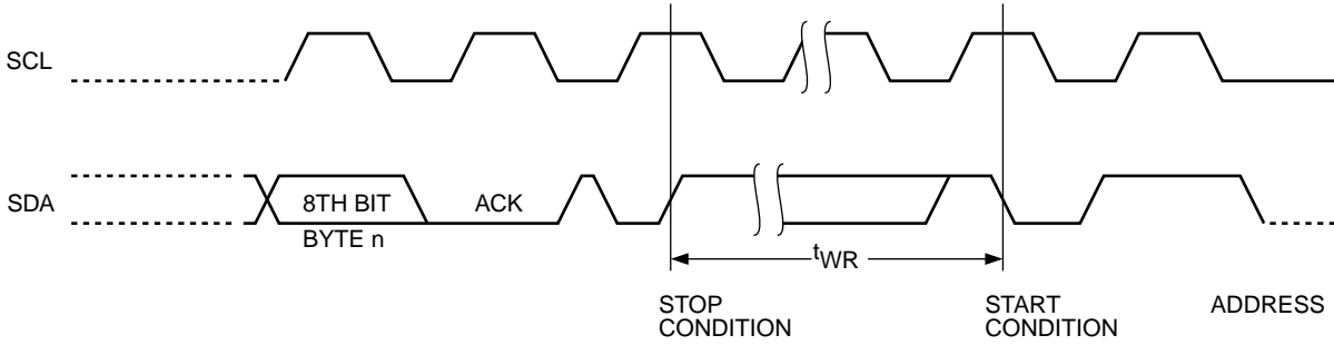
Figure 3. Start/Stop Condition
