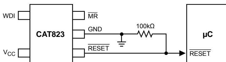
Figure 8. RESET Valid to 0 Volts V_{\text{CC}}
