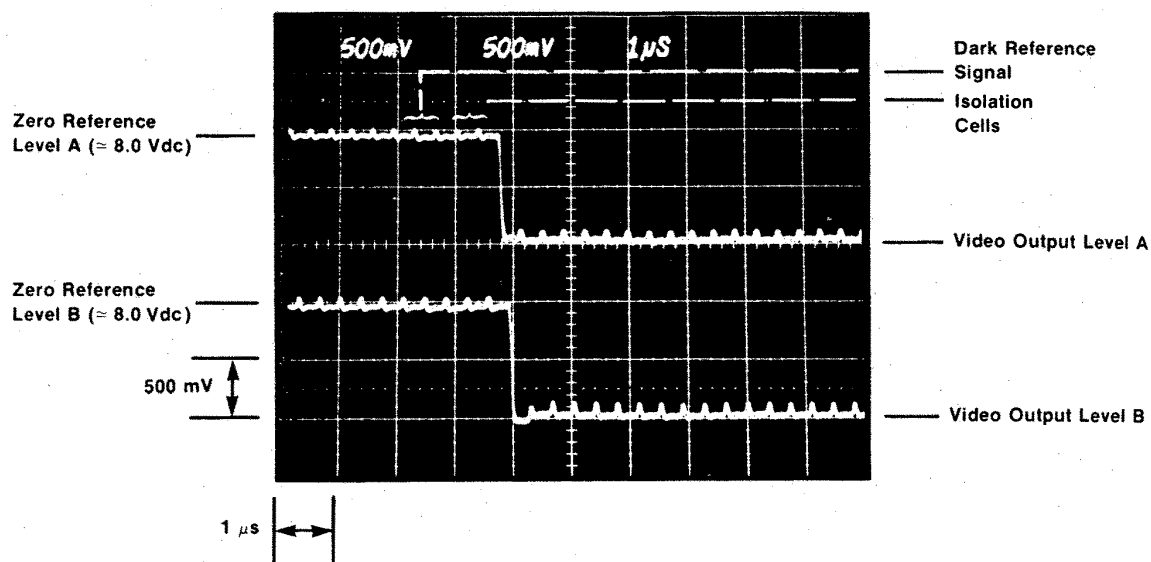
Start of One Scan Video Output
