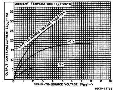
Fig. 3—Minimum n-channel output low (sink) current characteristics.
