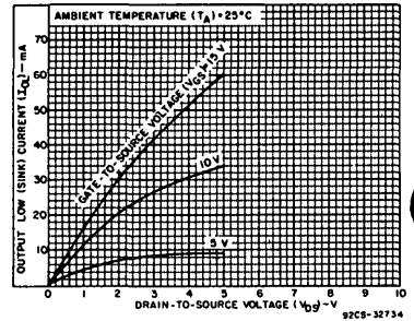
Fig. 2—Typical n-channel output low (sink) current characteristics.
