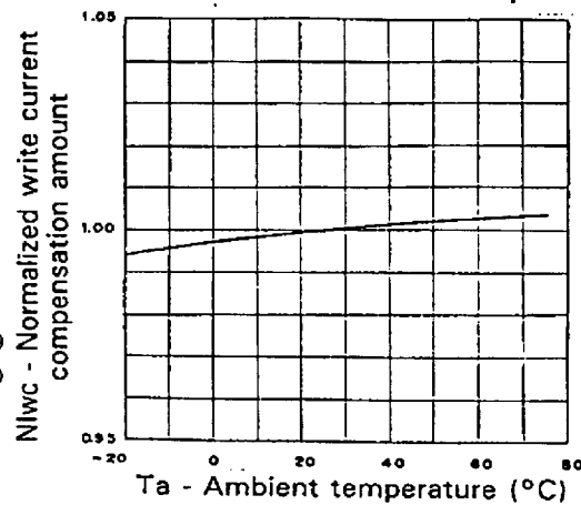
Normalized write current compensation amount vs. Ambient temperature
