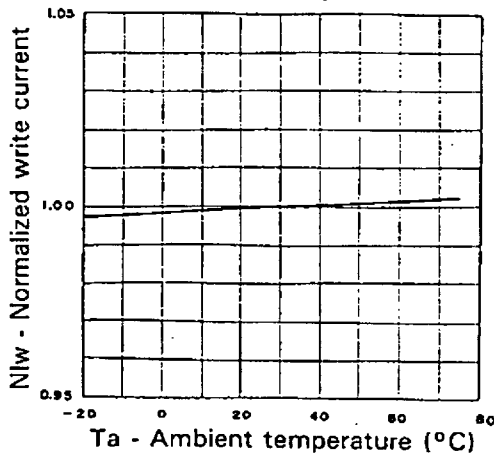
Normalized write current vs. Ambient temperature
