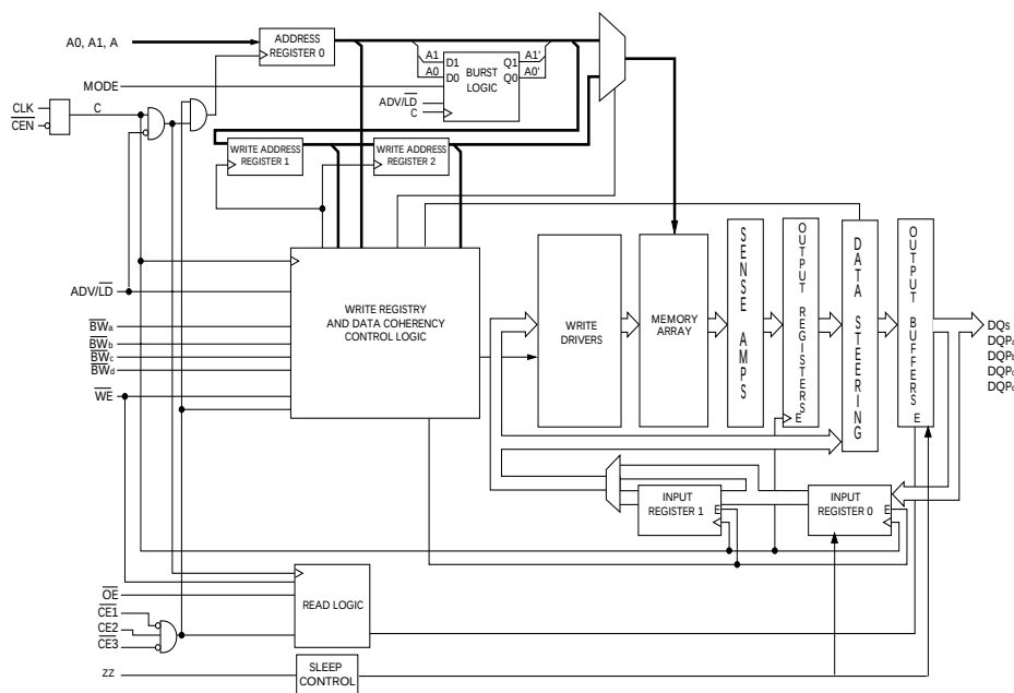
Logic Block Diagram—CY7C1354C (256K x 36)
